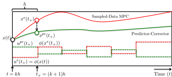
Fig. 2. Sketch of explicit and predictor-corrector sampled-data MPC schemes.
