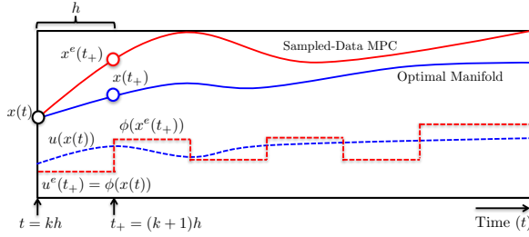
Fig. 1. Sketch of optimal solution manifold and sampled-data MPC.
